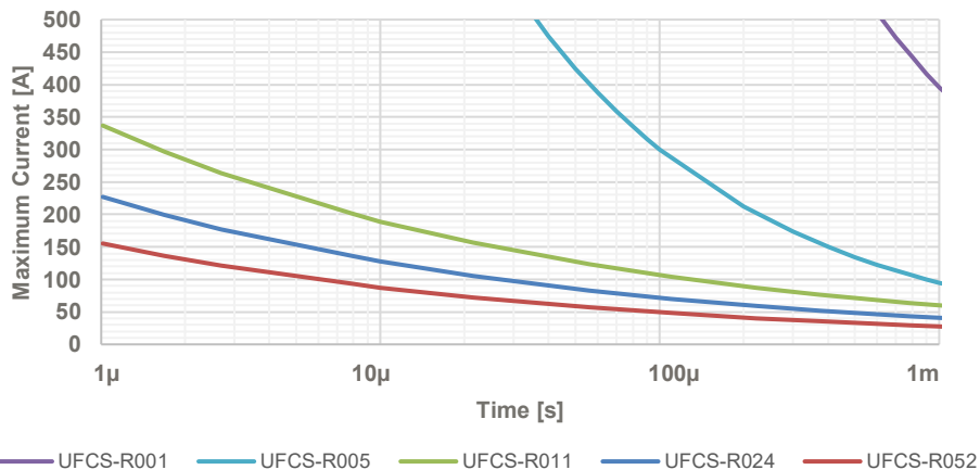
Maximum Current Ratings "Rectangular Pulse" UFCS-R0XX
