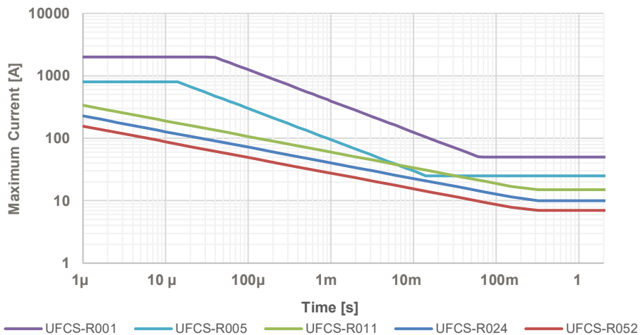
Maximum Current Ratings "Rectangular Pulse" UFCS-R0XX
