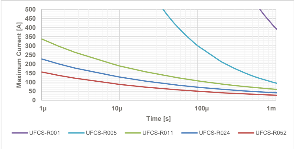
Maximum Current Ratings "Rectangular Pulse" UFCS-R0XX
